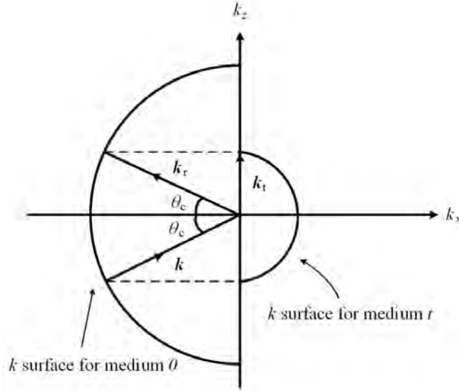
Figure 14.4: This figure (courtesy of J.A. Kong, Electromagnetic Wave Theory [31]), k in the figure is synonymous with \beta in our lecture notes, and x axis is the same as our z axis of our lecture notes.
