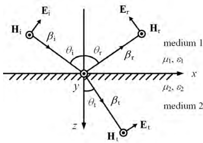
Figure 14.2: A similar schematic showing the reflection of the TM polarization wave impinging on a dielectric interface. The solution to this problem can be easily obtained by invoking duality principle.
