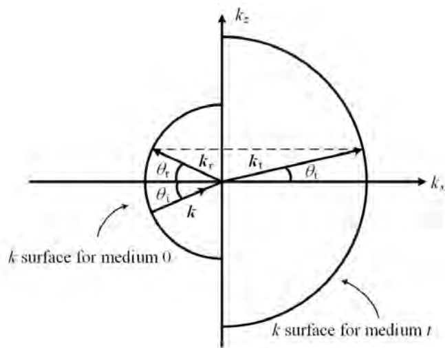
Figure 14.3: In this figure (courtesy of J.A. Kong, Electromagnetic Wave Theory [31]), k in the figure is synonymous with \beta in our lecture notes. Also, the x axis is equivalent to the z axis in the previous figure of our lecture notes.
